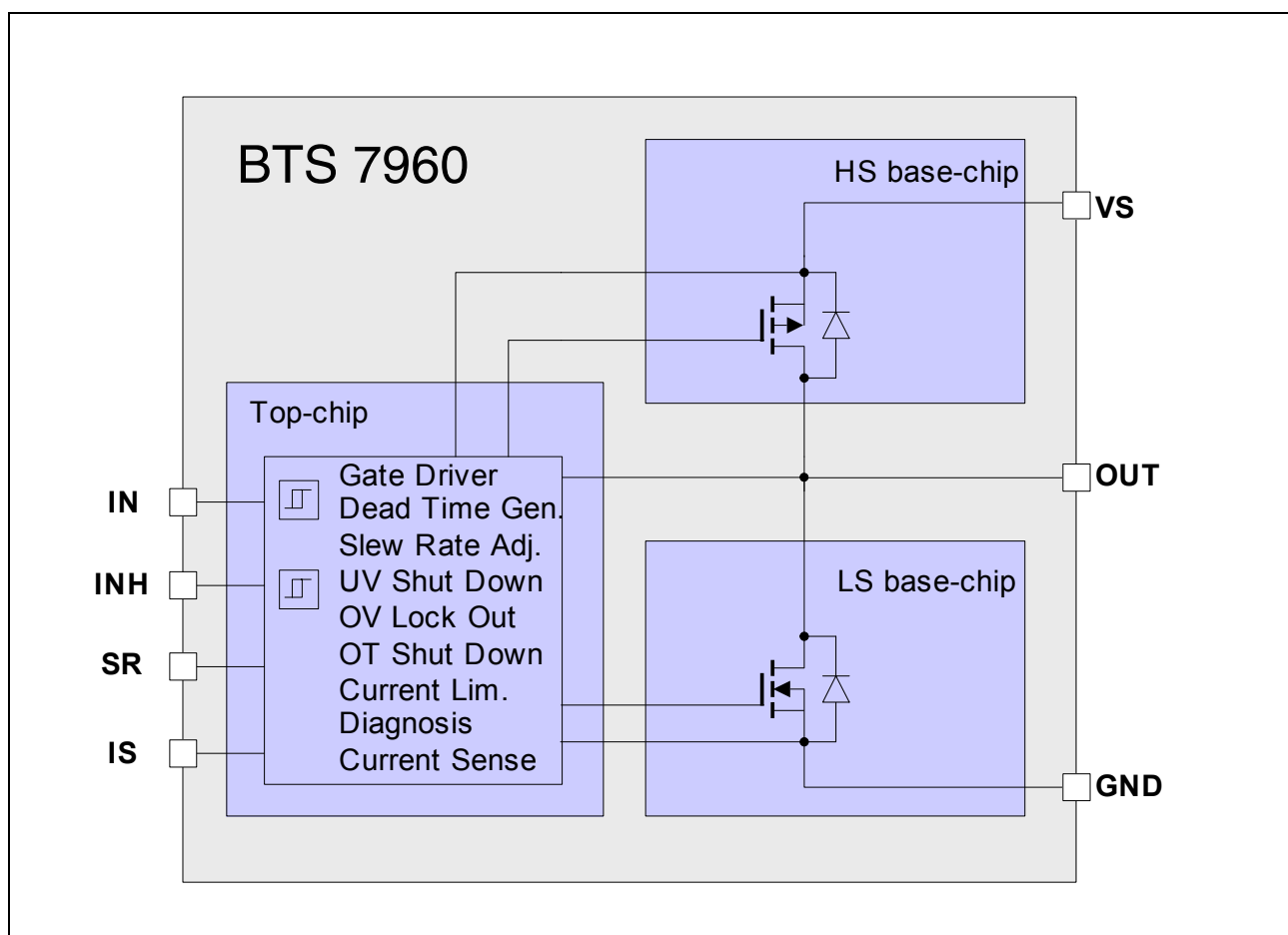
Figure 1 Block Diagram
