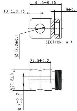
Piston rod eye option "5" Drawing no.: 0361138
