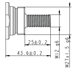
Back fixture option "5" Drawing no.: 0361126
