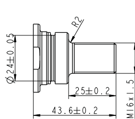
Back fixture option "6" Drawing no.: 0361247
