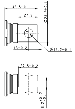
Back fixture option "7 & 8" Drawing no.: 0361140
