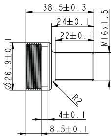
Piston rod eye option "4" Drawing no.: 0361135
