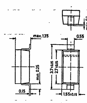
≈60A2 Diode Plastic Package Weight approx. 0.013 g
