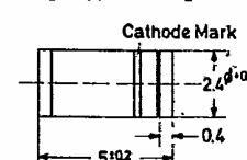
MELF Glass Case Weight approx. 0.25 g
