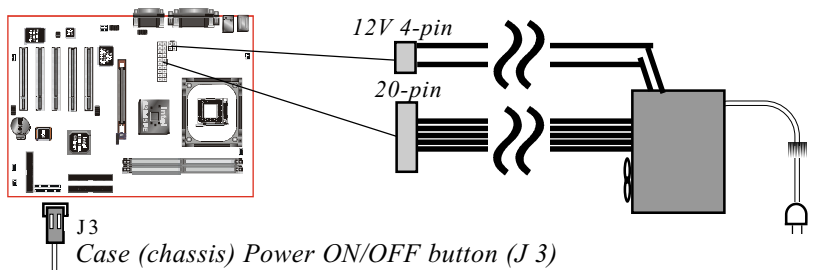
Figure 4: Simple ATX power ON/OFF controller
