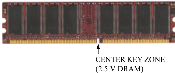
Figure 8 - DIMM notch
