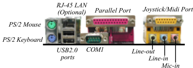
Figure 11 - I/O Ports
