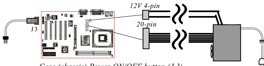
Figure 4: Simple ATX power ON/OFF controller
