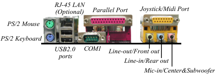
Figure 11 - I/O Ports
