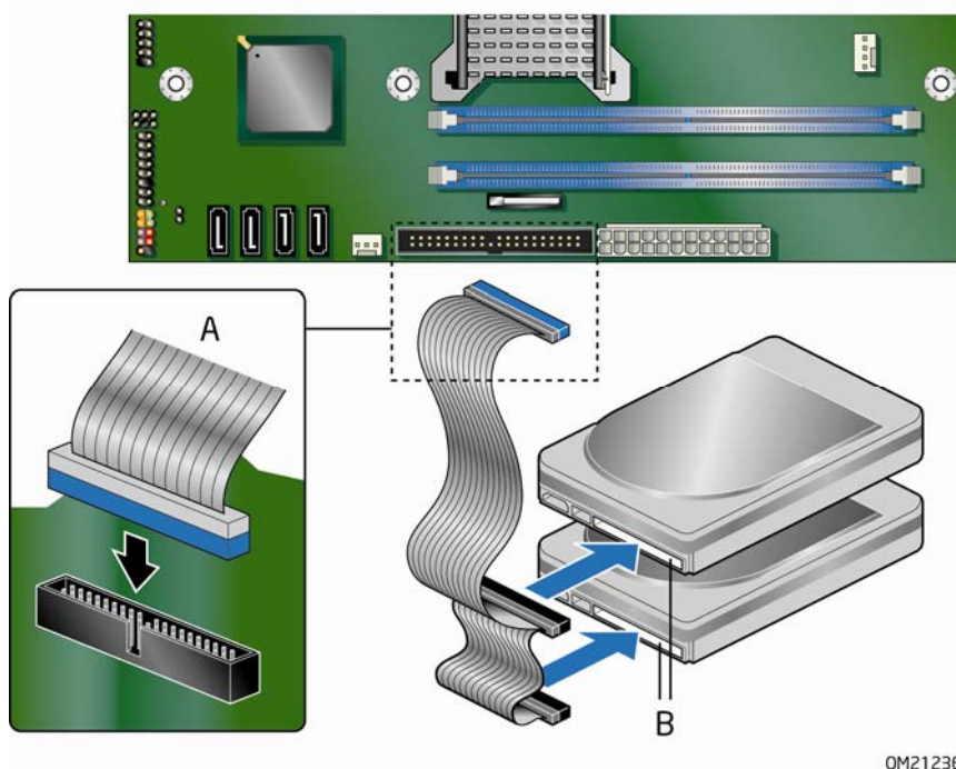
Figure 19. Connecting the IDE Cable
