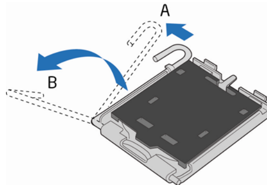
Figure 6. Lift the Socket Lever
