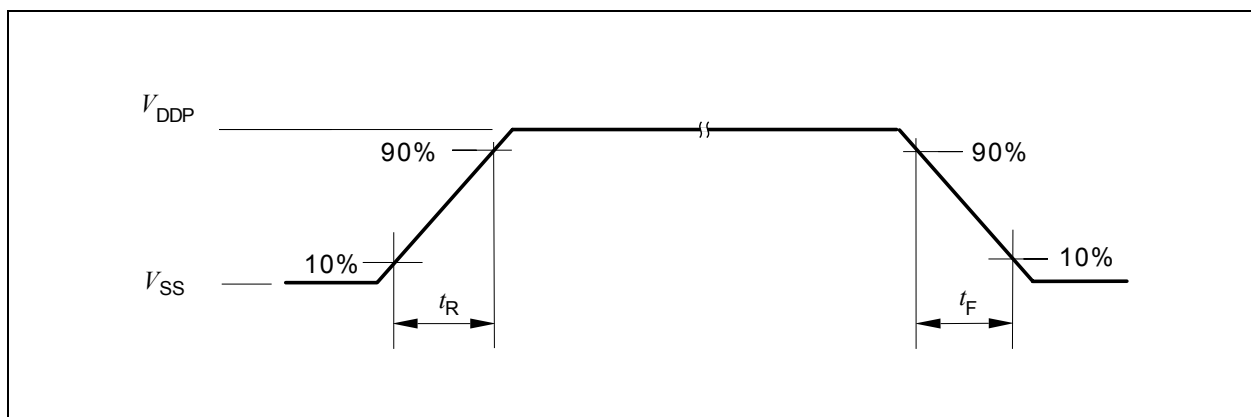
Figure 35 Rise/Fall Time Parameters
