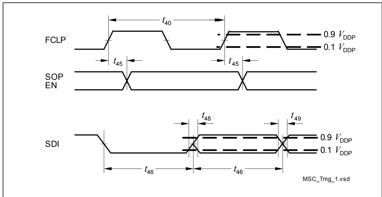
Figure 4-14 MSC Interface Timing
