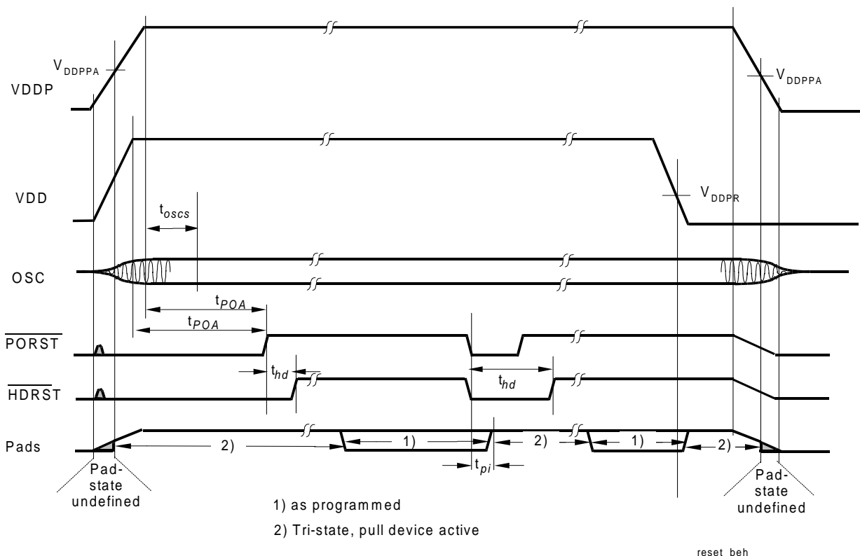
Figure 4-11 Power, Pad and Reset Timing
