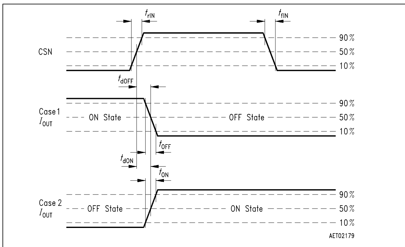
Figure 13 Turn OFF/ON Time
