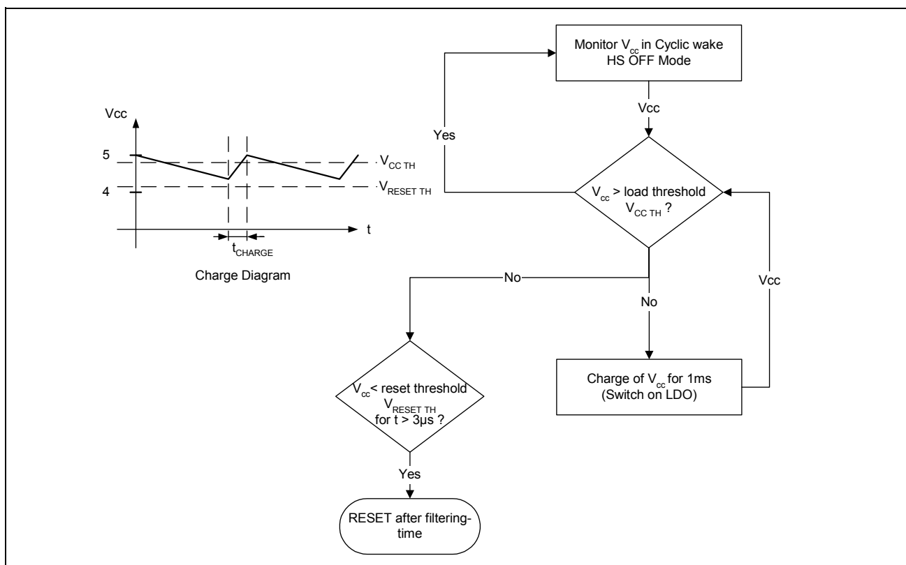
Figure 6 LDO activation flowchart for the cyclic wake HS OFF mode
