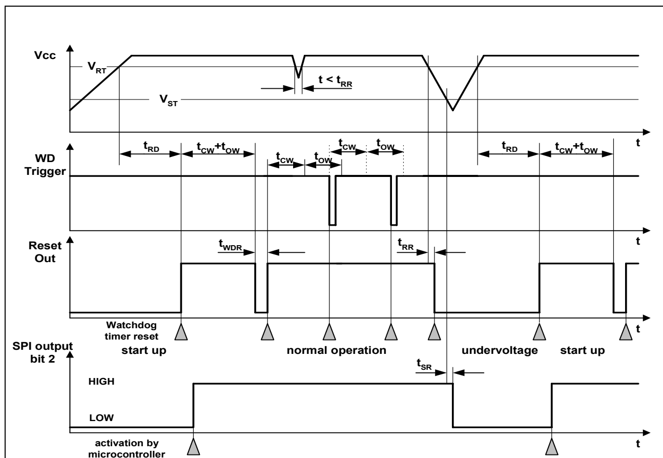
Figure 20 Reset Timing Diagram
