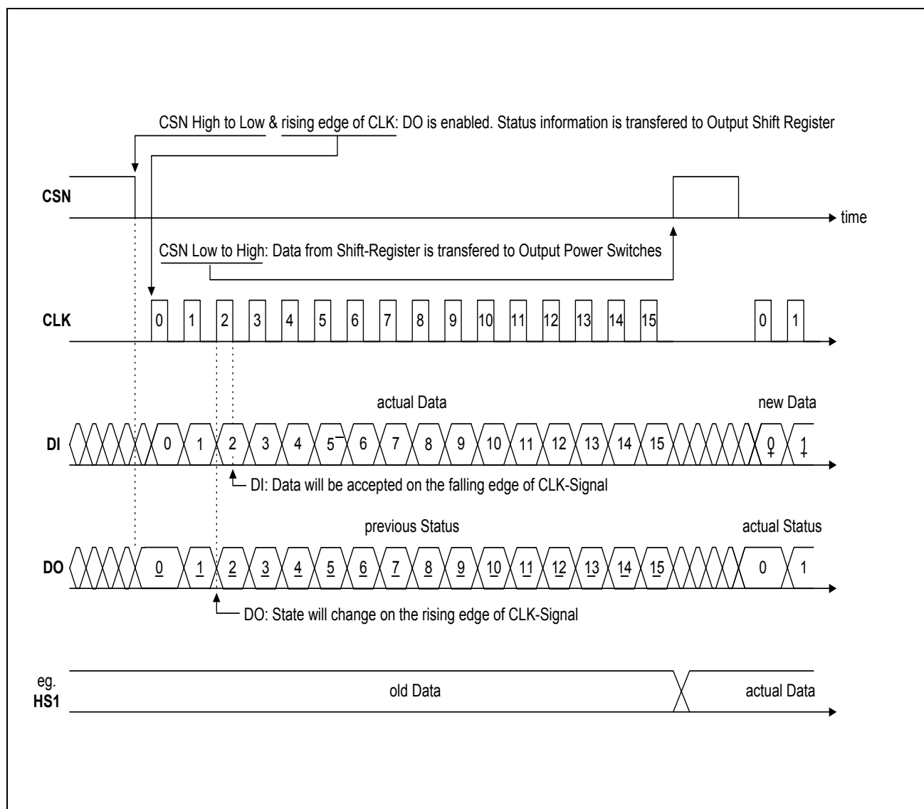
Figure 11 Data Transfer Timing
