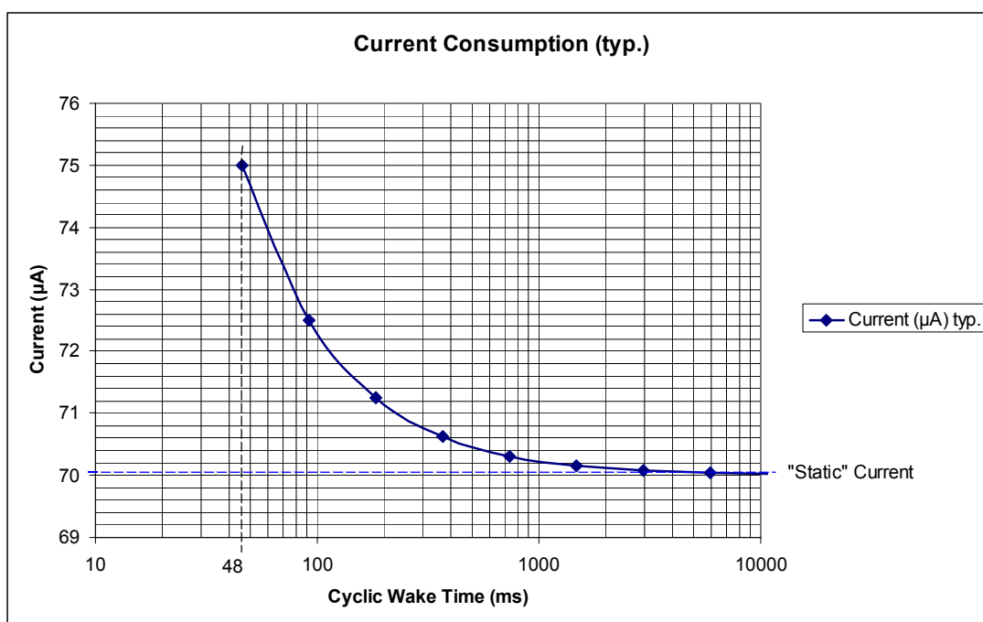
Figure 21 Current Consumption during Cyclic Wake Mode
