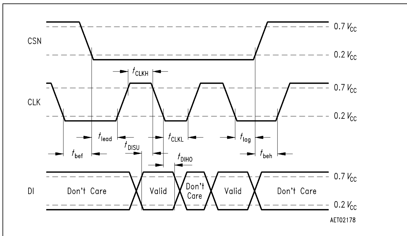
Figure 12 SPI-Input Timing
