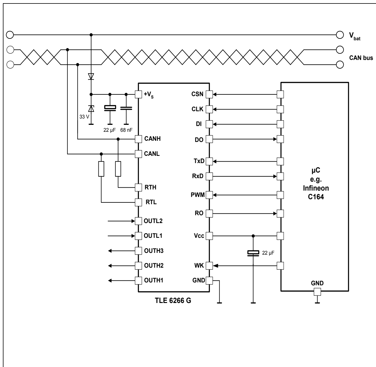
Figure 23 Application Circuit
