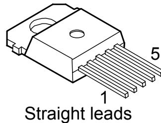
TO-218AB/5
