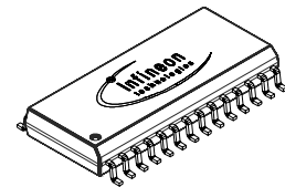
P-DSO-28-18 Enhanced Power
