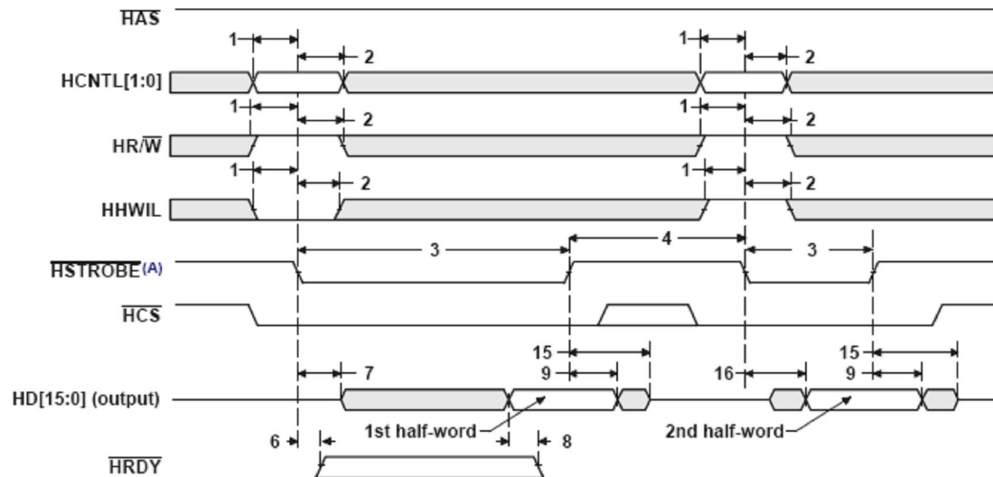
图5-38 HPI16读时序 ( \overline{\text{HAS}} 没用, 强制为高电平)
