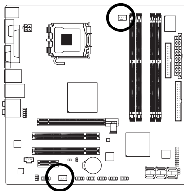
1 CPU_FAN / SYS_FAN
