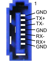
SATA_1/2/3/4
