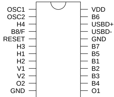
24 Pin Package
