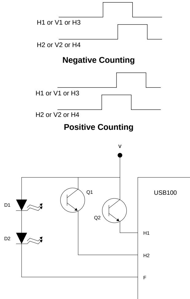
Schematic 1: Roller Mode of Operation
