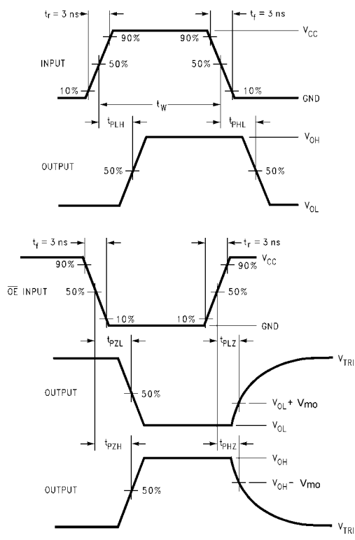
FIGURE 2. AC Waveforms
