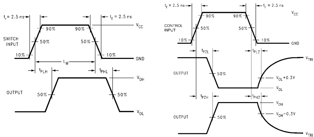
FIGURE 2. AC Waveforms
