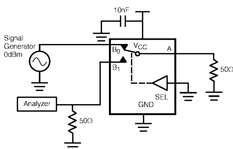
FIGURE 6. Crosstalk
