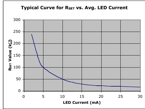
Figure 2. The typical curve of R_{SET} vs. LEDs average current.
