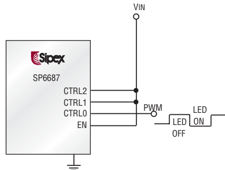
Figure 4. Typical application circuit for PWM dimming when driving 4 LEDs.
