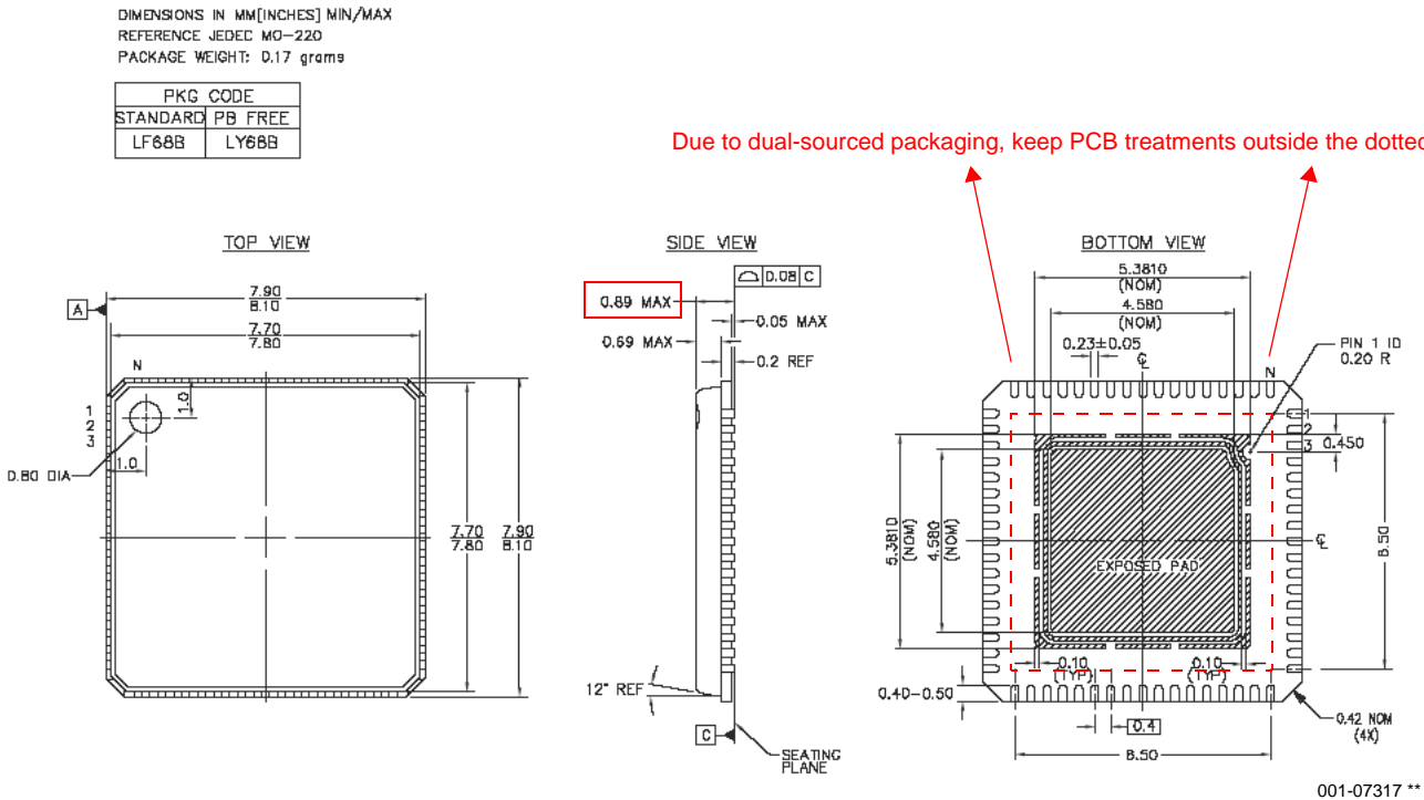
Figure 4-2. 68-Lead (8x8 mm x 0.89 mm) QFN
