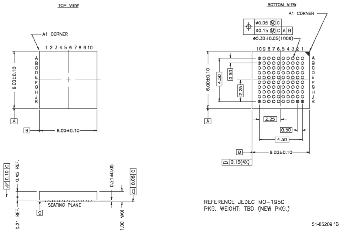
Figure 4-4. 100-Ball (6x6 mm) VFBGA
