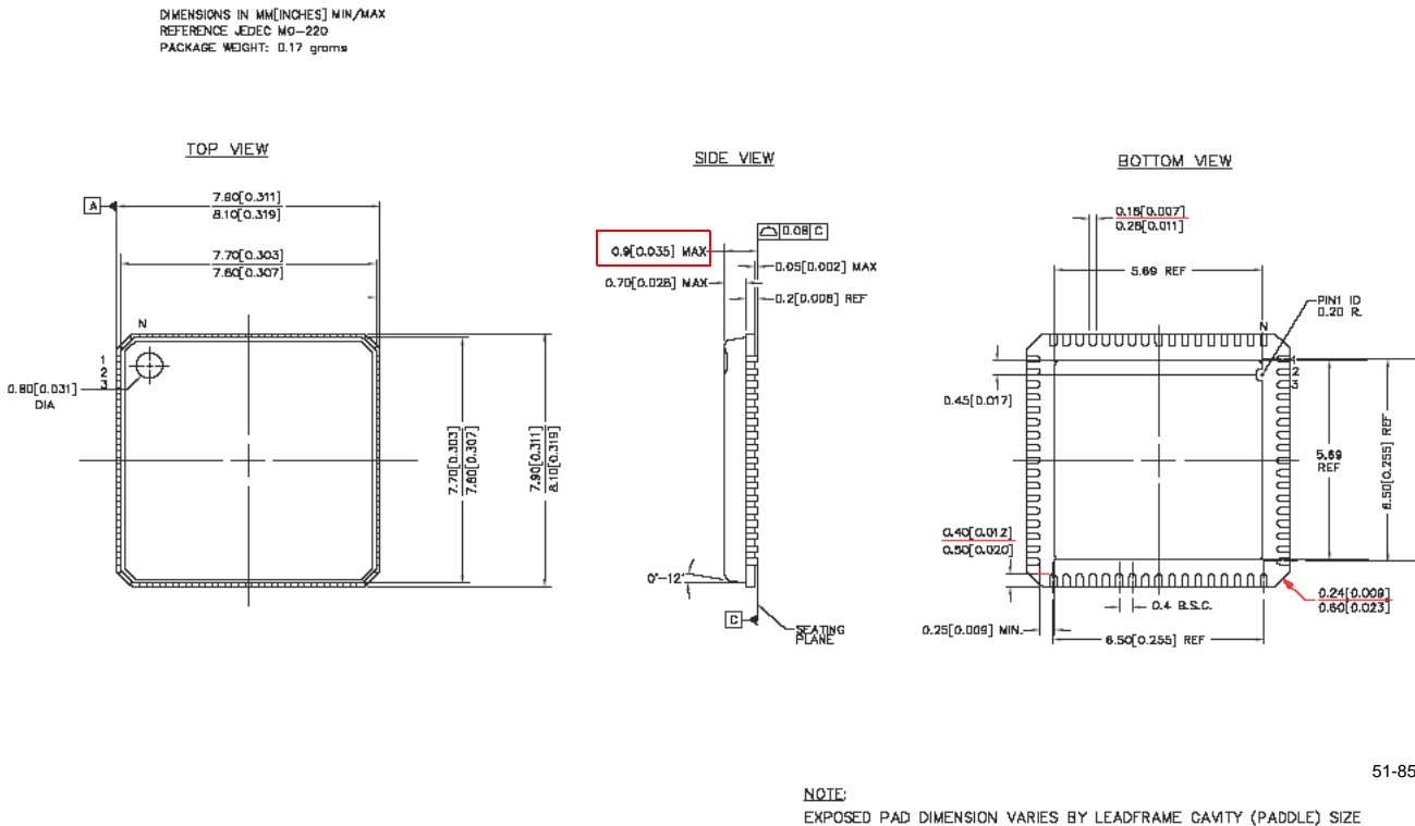
Figure 4-3. 68-Lead (8x8 mm x 0.9 mm) QFN
