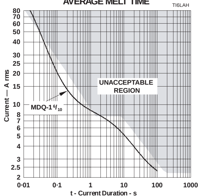
Figure 17. MDQ-1 6/_{10} Current-Time
