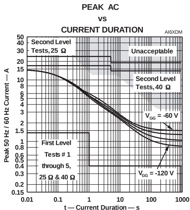
Figure 19. TISP61089B Overlay
