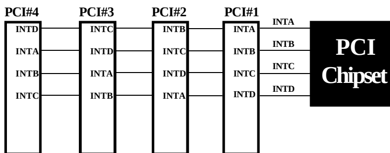
Figure 4-7 The Combination of PCI INT# lines
