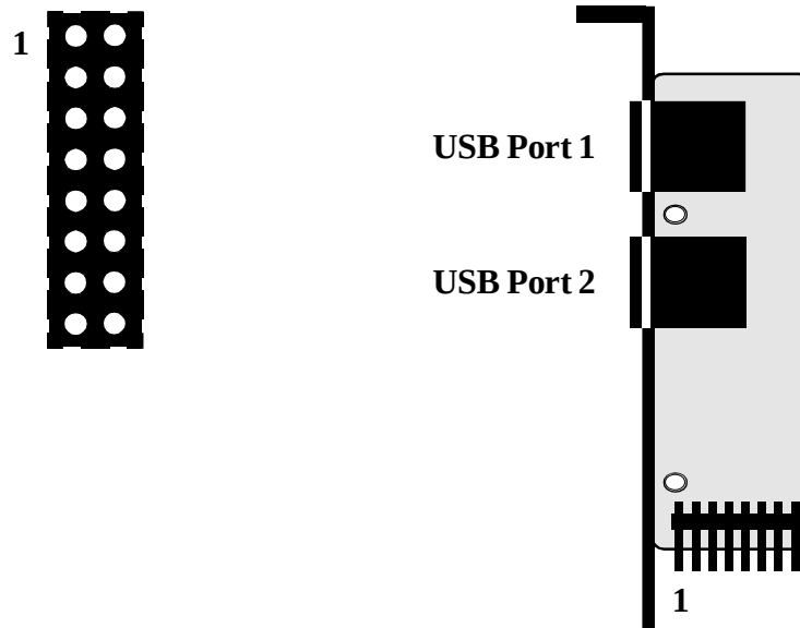
Figure 5-2 USB Port Adapter
