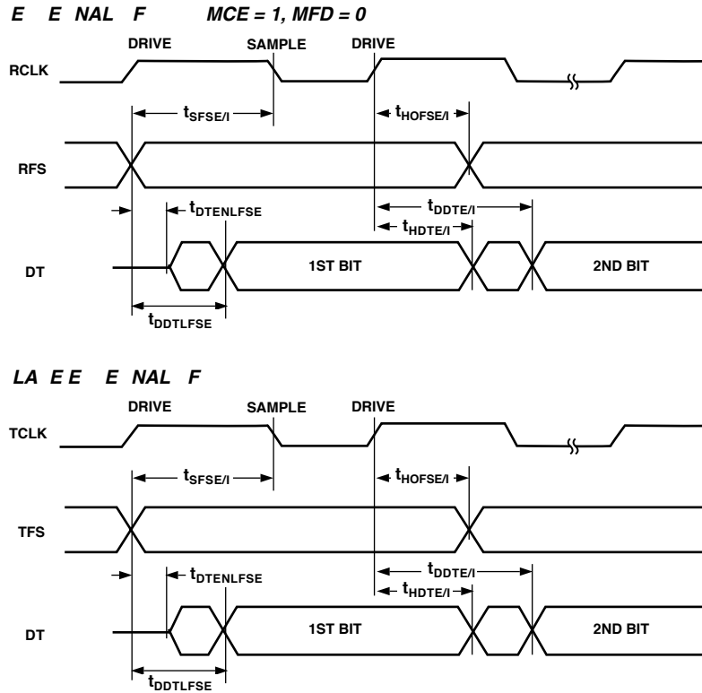
Figure 21. External Late Frame Sync (Frame Sync Setup < t_{sCLK}/2 )
