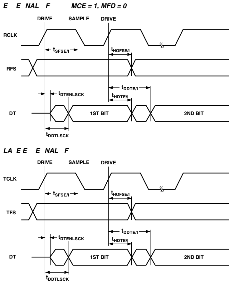
Figure 22. External Late Frame Sync (Frame Sync Setup > t_{sCLK}/2 )
