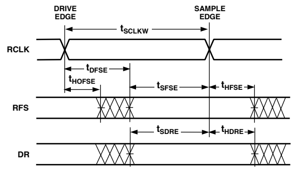
DATA ACQUISITION IN SERIAL CLOCK
