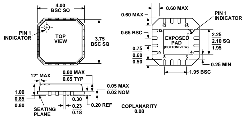
Figure 28. 16-Lead Lead Frame Chip Scale Package [LFCSP_VQ] 4 mm × 4 mm Body, Very Thin Quad (CP-16-4) Dimensions shown in millimeters
