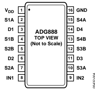
Figure 4. 16-Lead TSSOP (RU-16)
