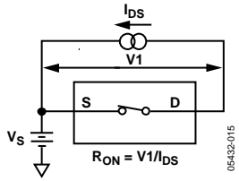
Figure 16. On Resistance
