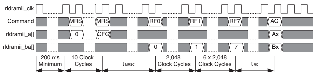
Figure 2–11. RLDRAM II Initialization Sequence
