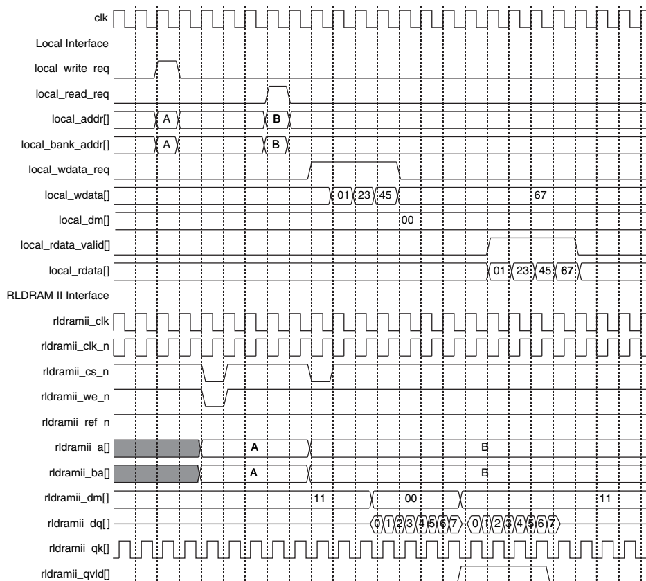
Figure 2–15. Read Following a Write
