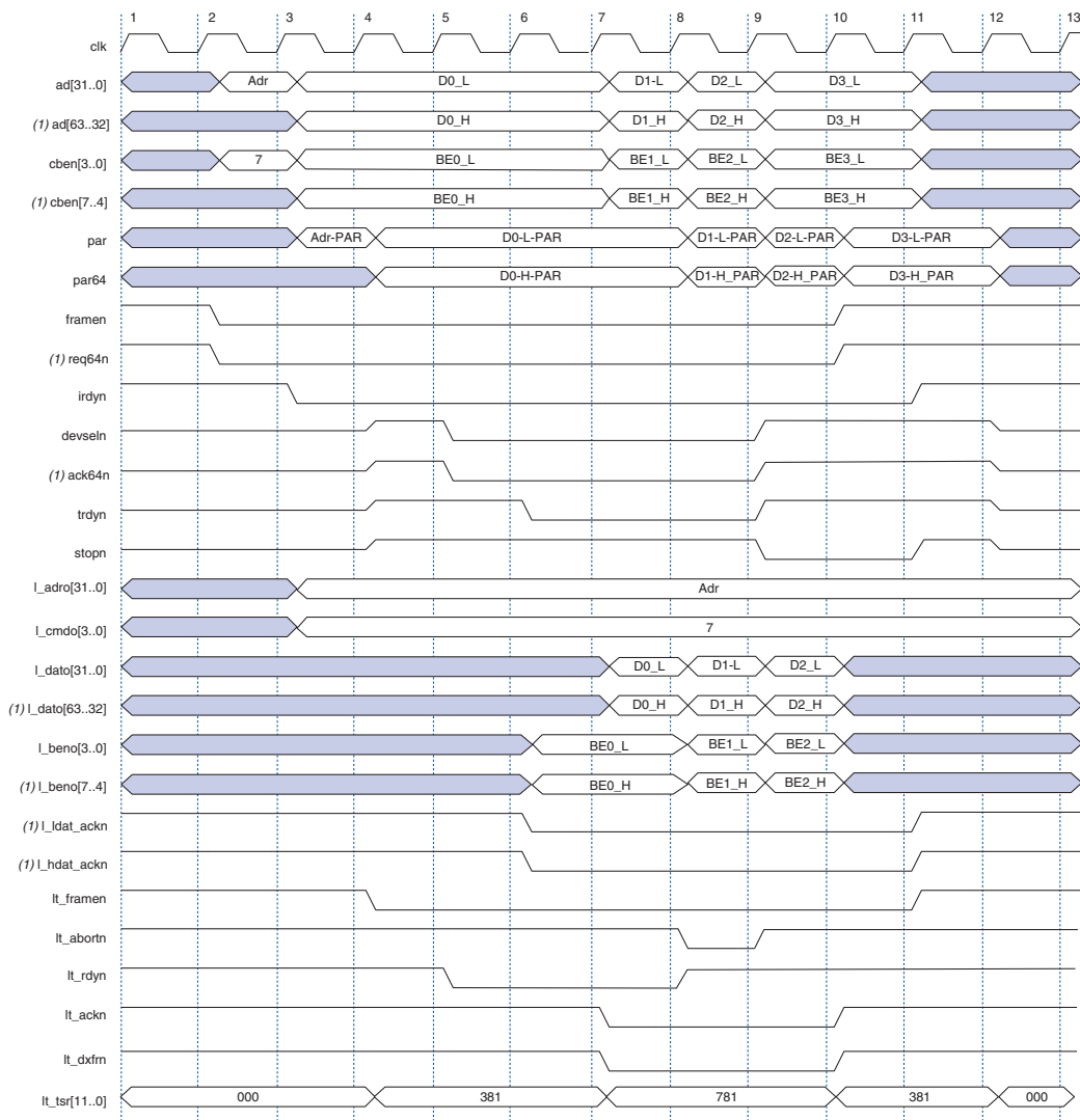
Figure 3–30. Target Abort
