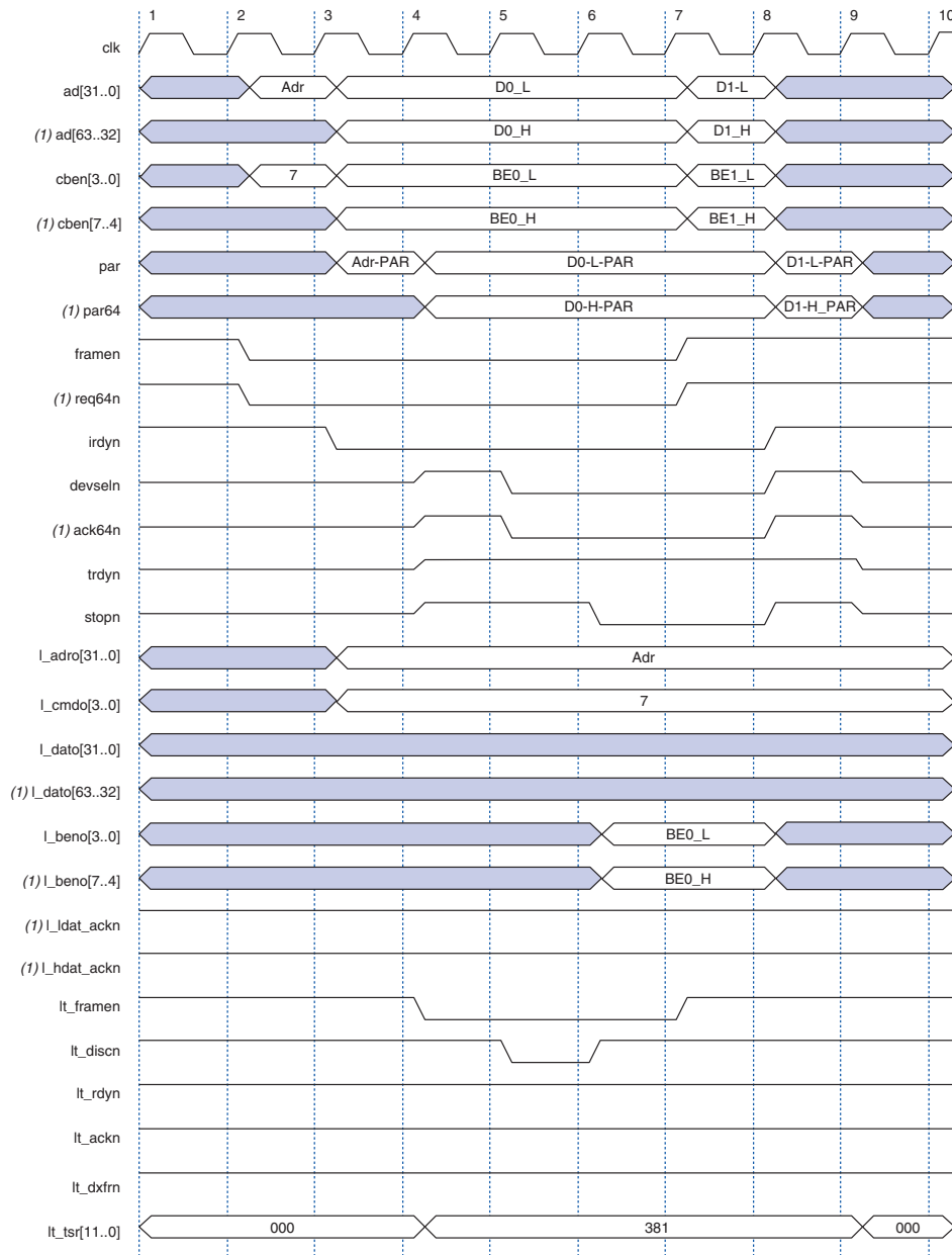
Figure 3–23. Target Retry
