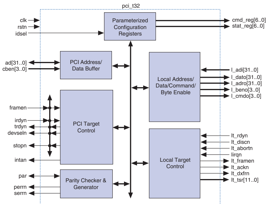
Figure 3–4. pci_t32 Functional Block Diagram
