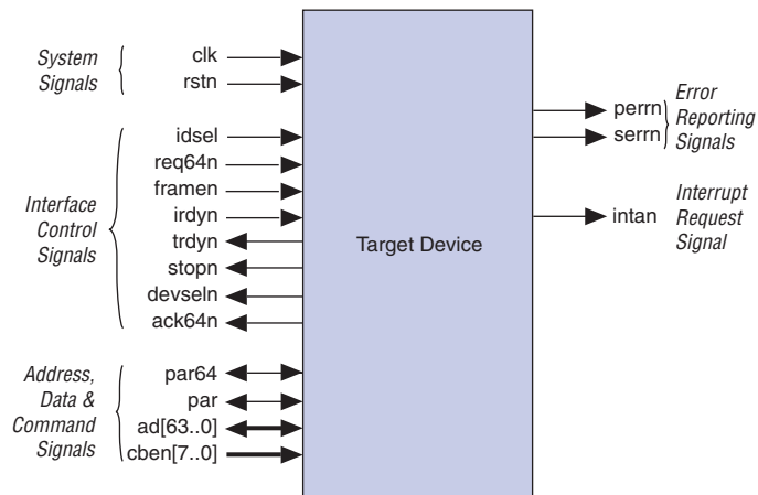
Figure 3–5. Target Device Signals
