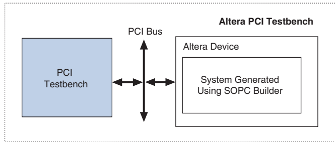
Figure 8–3. Typical Verification Environment Using the PCI Testbench
