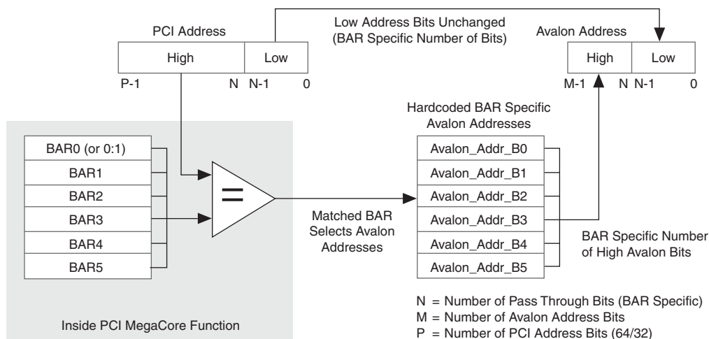
Figure 7–8. PCI-to-Avalon Address Translation
