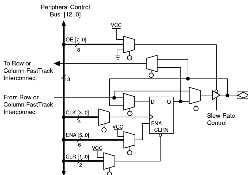
Figure 10. MAX 9000 IOC
