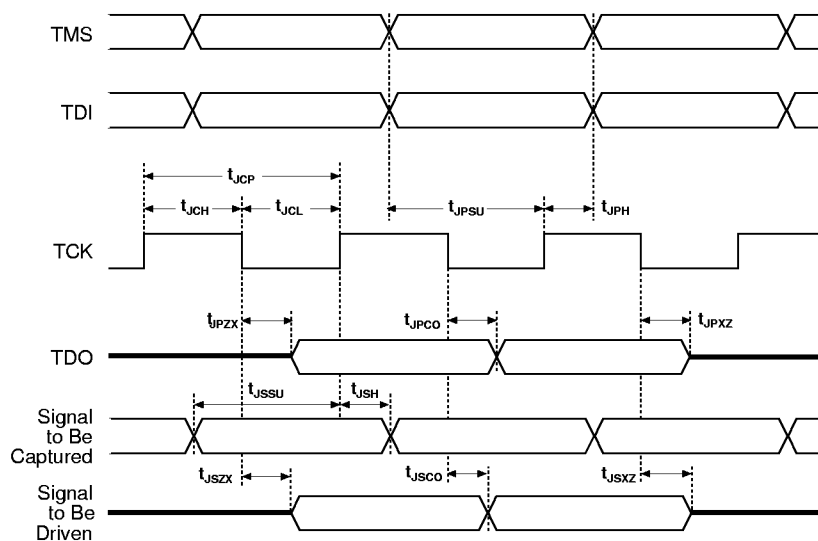
Figure 11. MAX 9000 JTAG Waveforms
