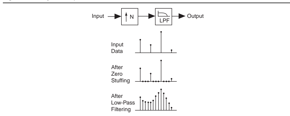
Figure 4-7. Signal Interpolation
