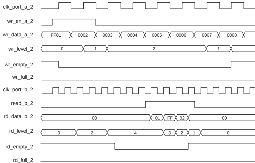
Figure 9. Writing 16-bit words and reading 8-bit words
