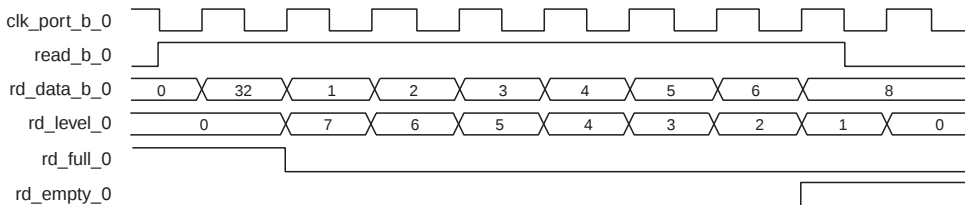
Figure 7. Using read_b_n as a Read Request
