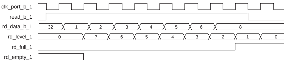
Figure 8. Using read_b_n as a Read Acknowledge
