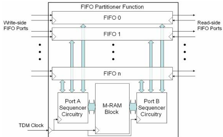
Figure 2. Detailed view of FIFO Partitioner function
