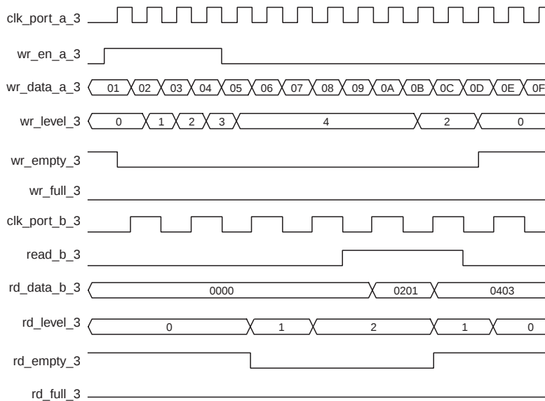
Figure 10. Writing 8-bit words and reading 16-bit words
