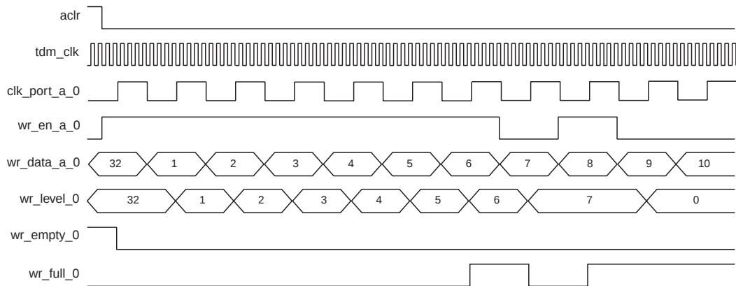
Figure 6. Initializing and Writing to a FIFO
