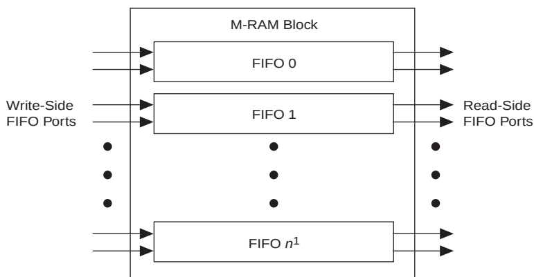
Figure 1. User's View of a FIFO Partitioner Function Note (1)
