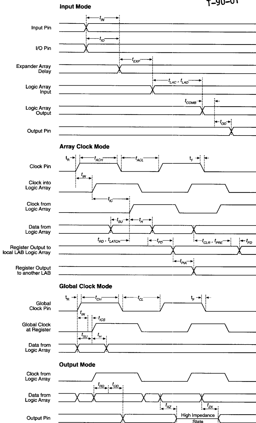
Figure 7. Switching Waveforms
