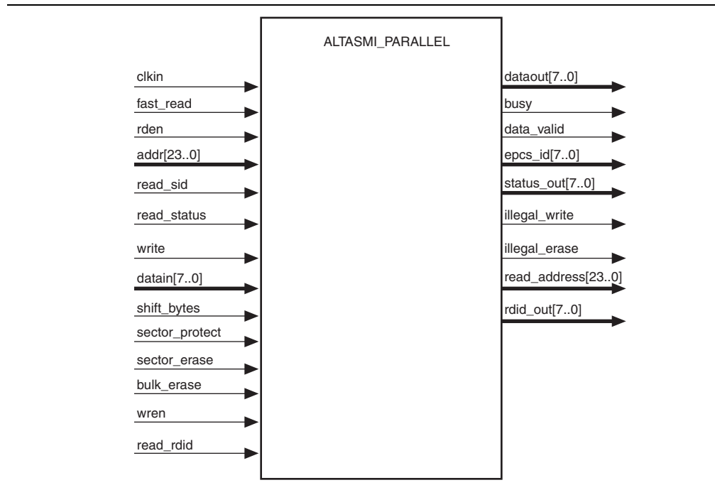
Figure 1. ALTASMI_PARALLEL Block Diagram
