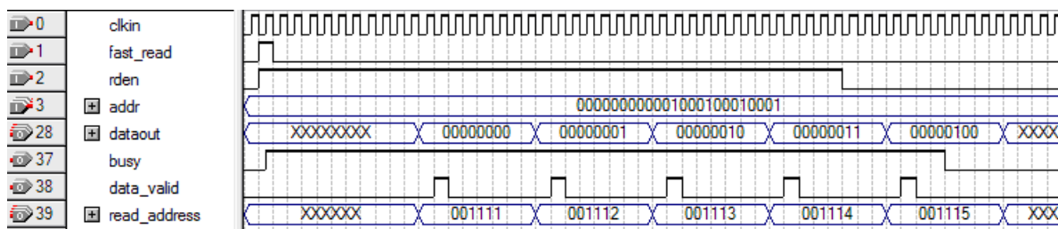
Figure 7. Fast Reading Multiple-Byte (Note 1)
