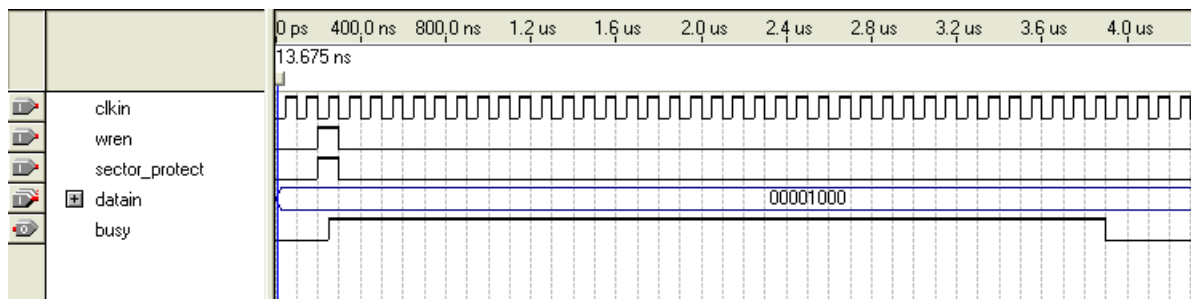
Figure 14. Protecting a Sector
