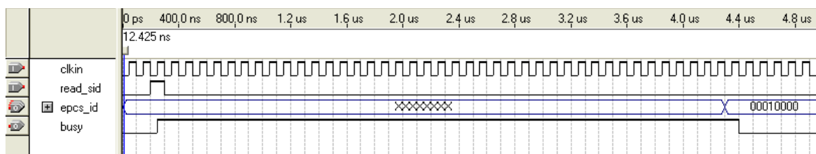
Figure 4. Reading Silicon ID (Note 1)
