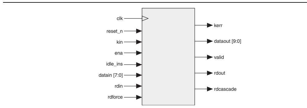
Figure 3–3. Encoder
