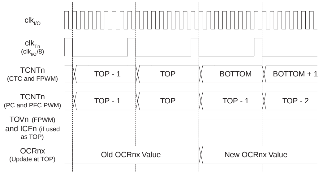
Figure 44. T/C 时序图，预分频器为 f_{clk\_I/O}/8
