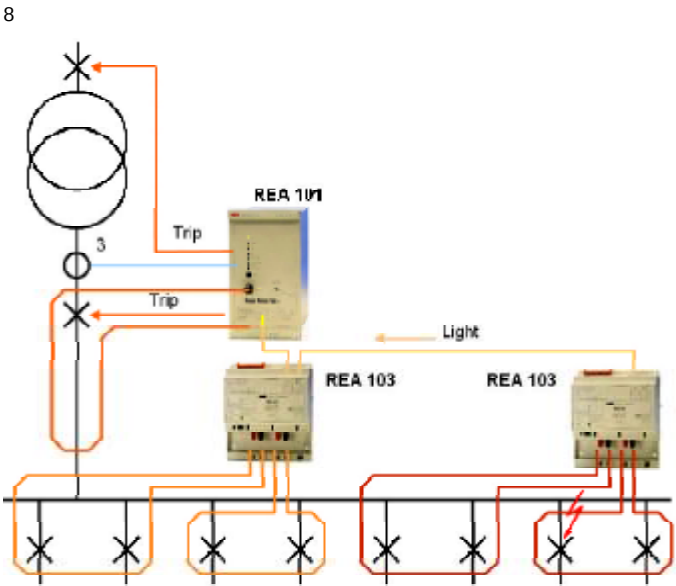
8 REA101、REA103 典型的配置方案
