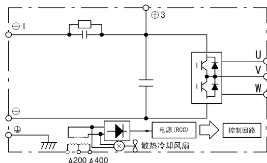
CIMR-G5AE055~E160形 (55~160kW)
