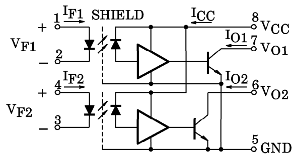
SCHEMATIC
