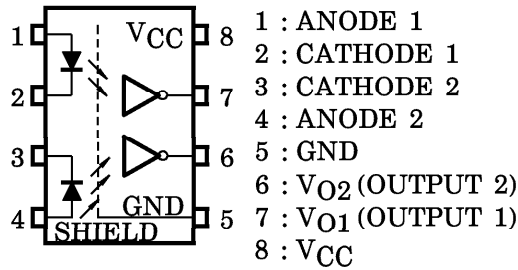
SCHEMATIC
