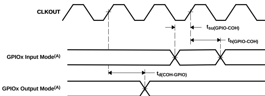
Figure 5-31. GPIOx (A) Timings
