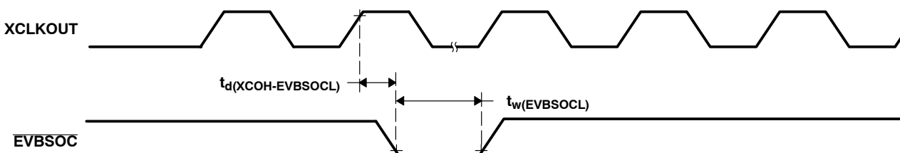
Figure 6–16. \overline{EVBSOCL} Timing
