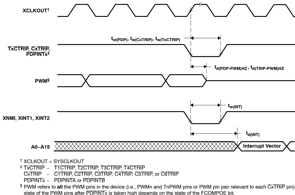
Figure 6-17. External Interrupt Timing
