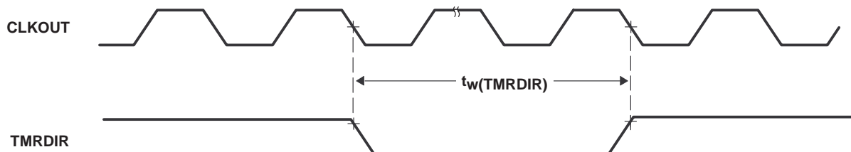
Figure 27. Capture/TMRDIR Timing
