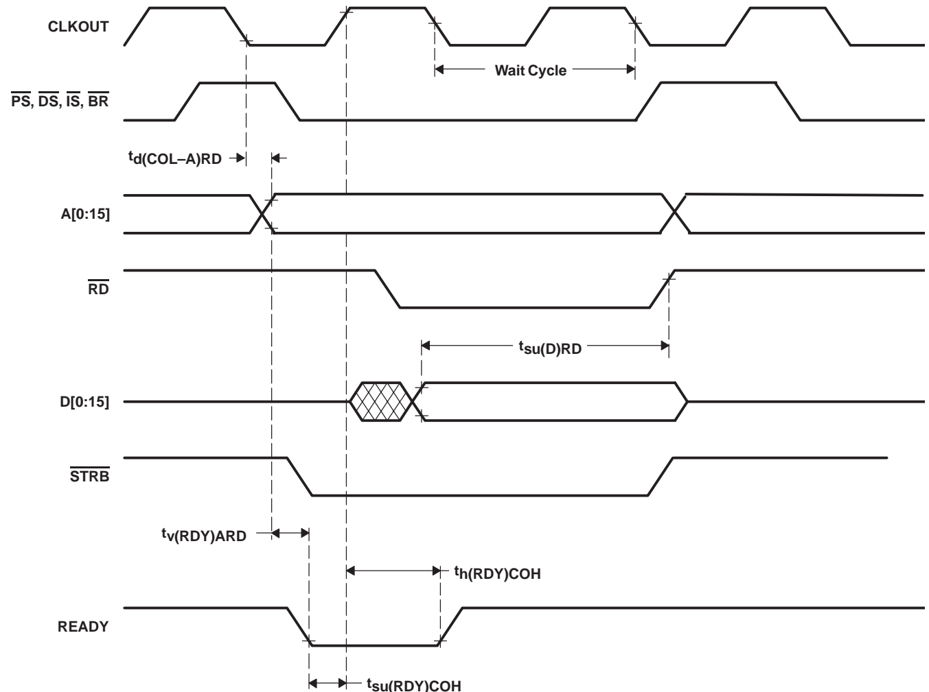
Figure 38. Ready-on-Read Timings
