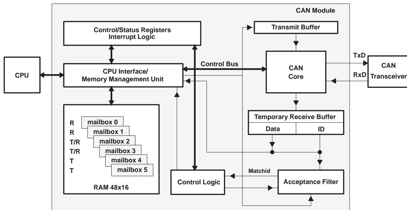
Figure 11. CAN Module Block Diagram
