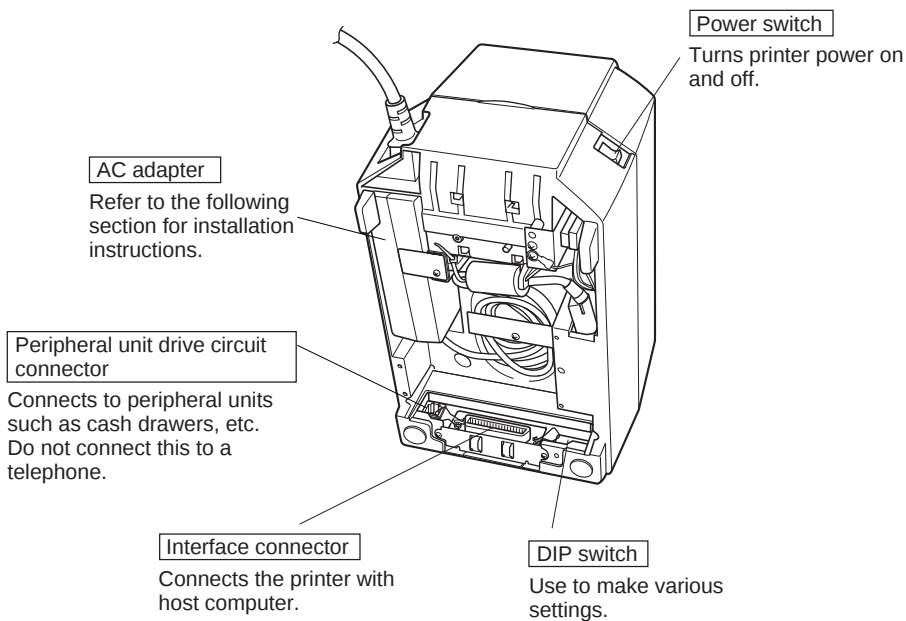
Fig. 3-1 External view of the printer (SP2300 type)
