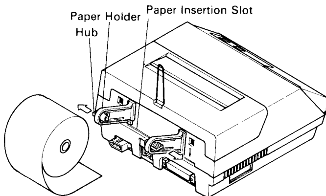
Figure 4-4. Paper Insertion (1)
