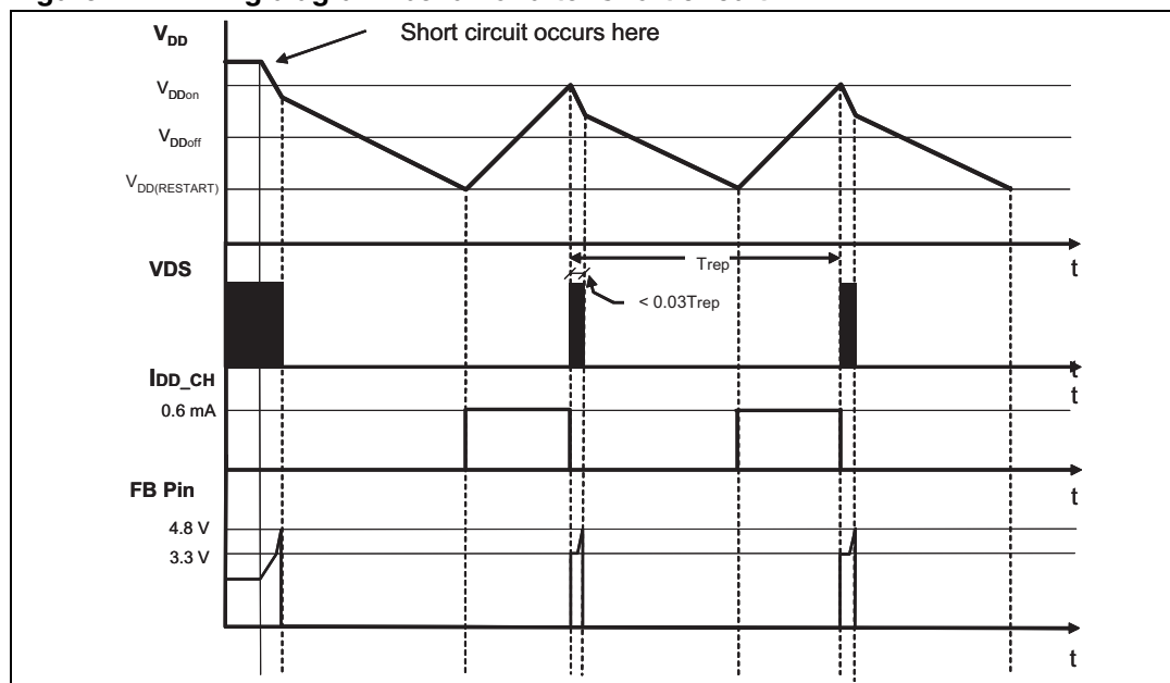
Figure 21. Timing diagram: behavior after short circuit
