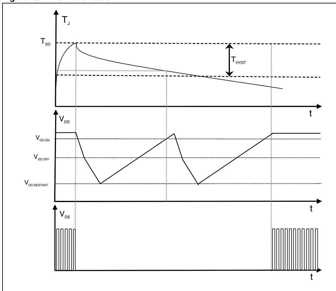
Figure 15. Thermal shutdown
