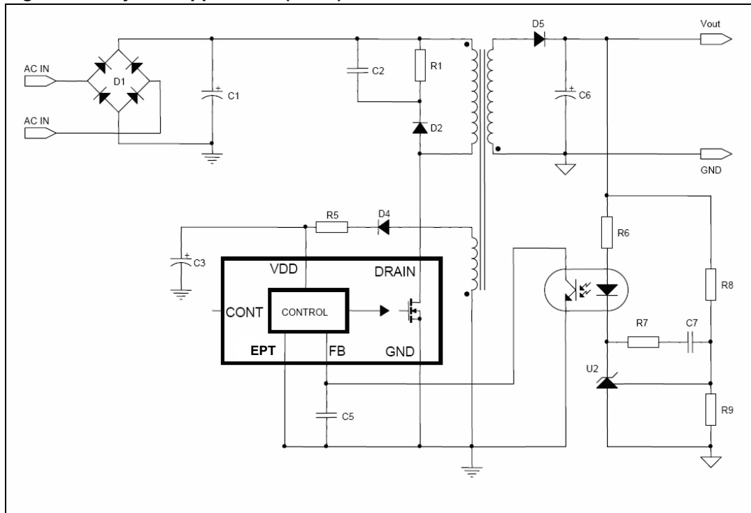
Figure 16. Flyback application (basic)
