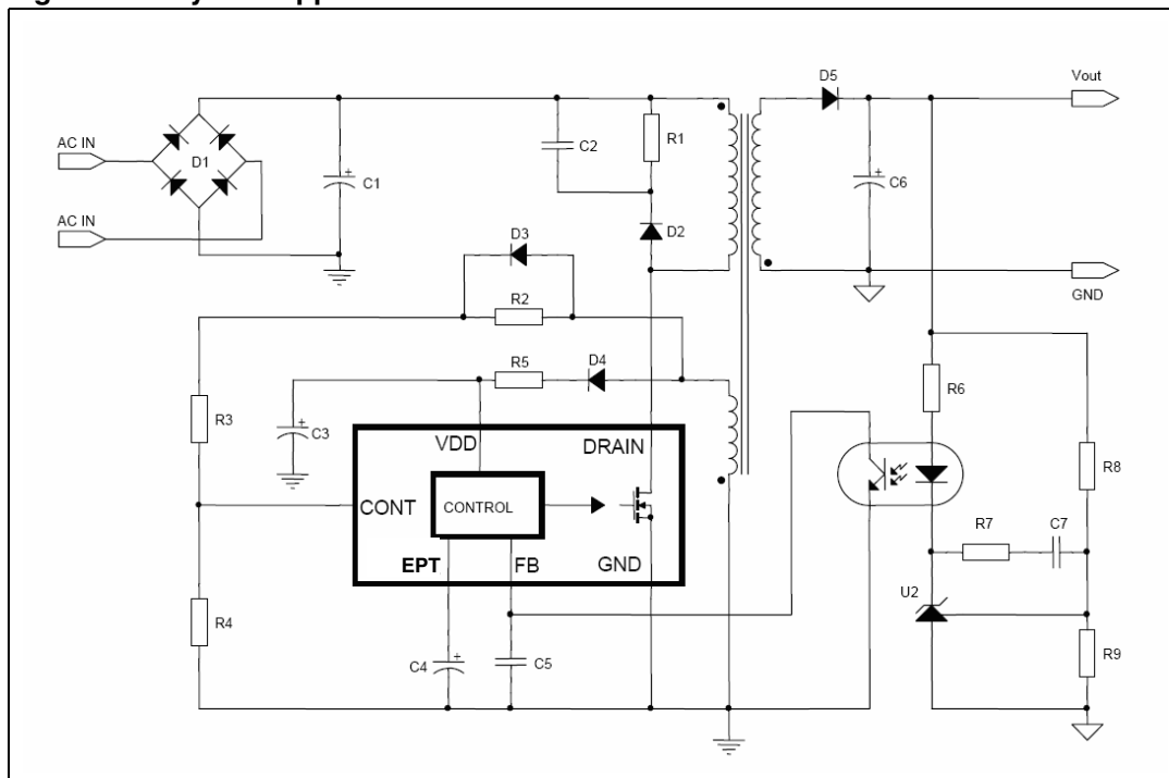
Figure 17. Flyback application
