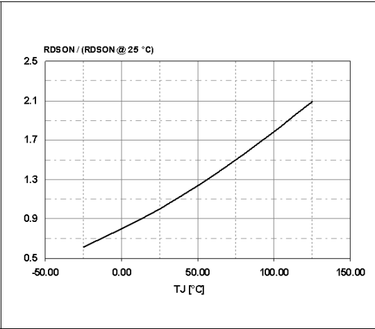
Figure 13. Power MOSFET on-resistance vs T_J
