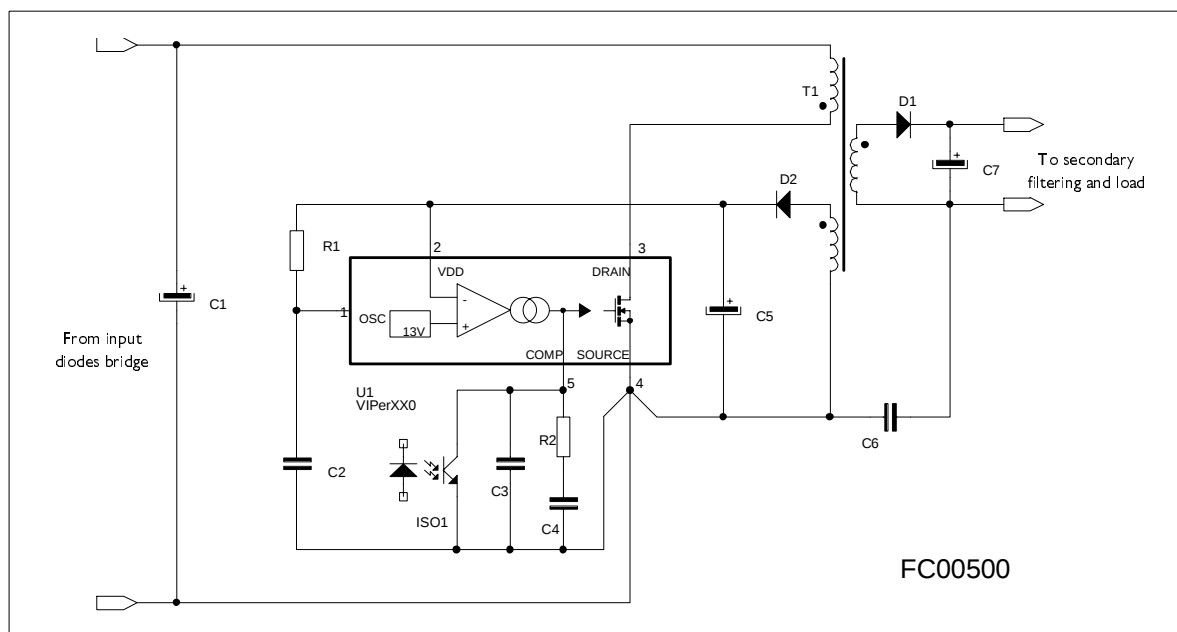
Figure 23: Recommended Layout
