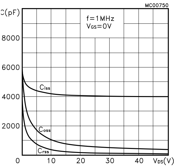
Figure 10: Capacitance Variations
