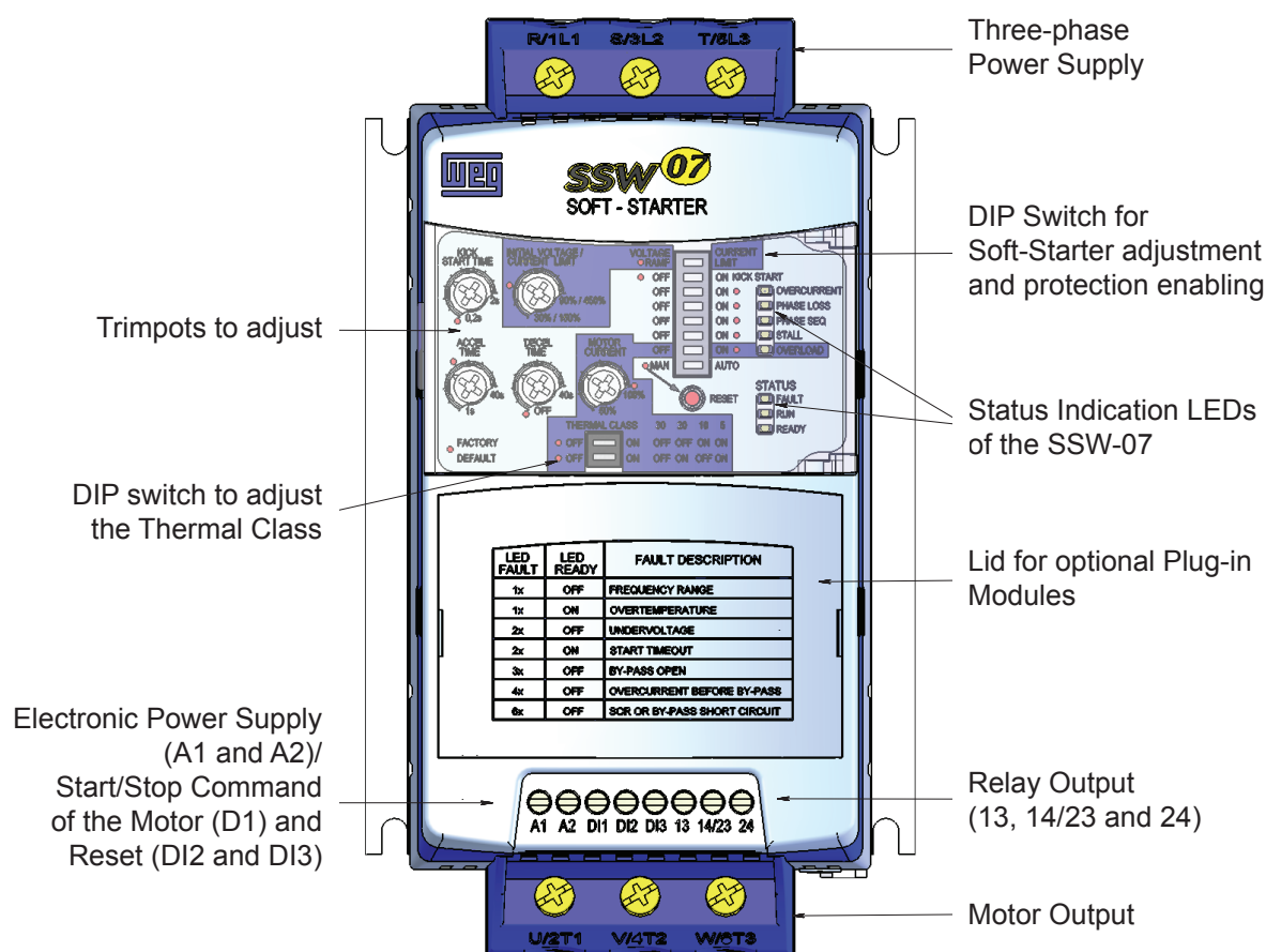
Figure 2.1 - Frontal view of the SSW-07
