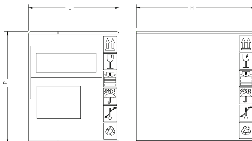
Figure 2.5 - Dimensions of the package
