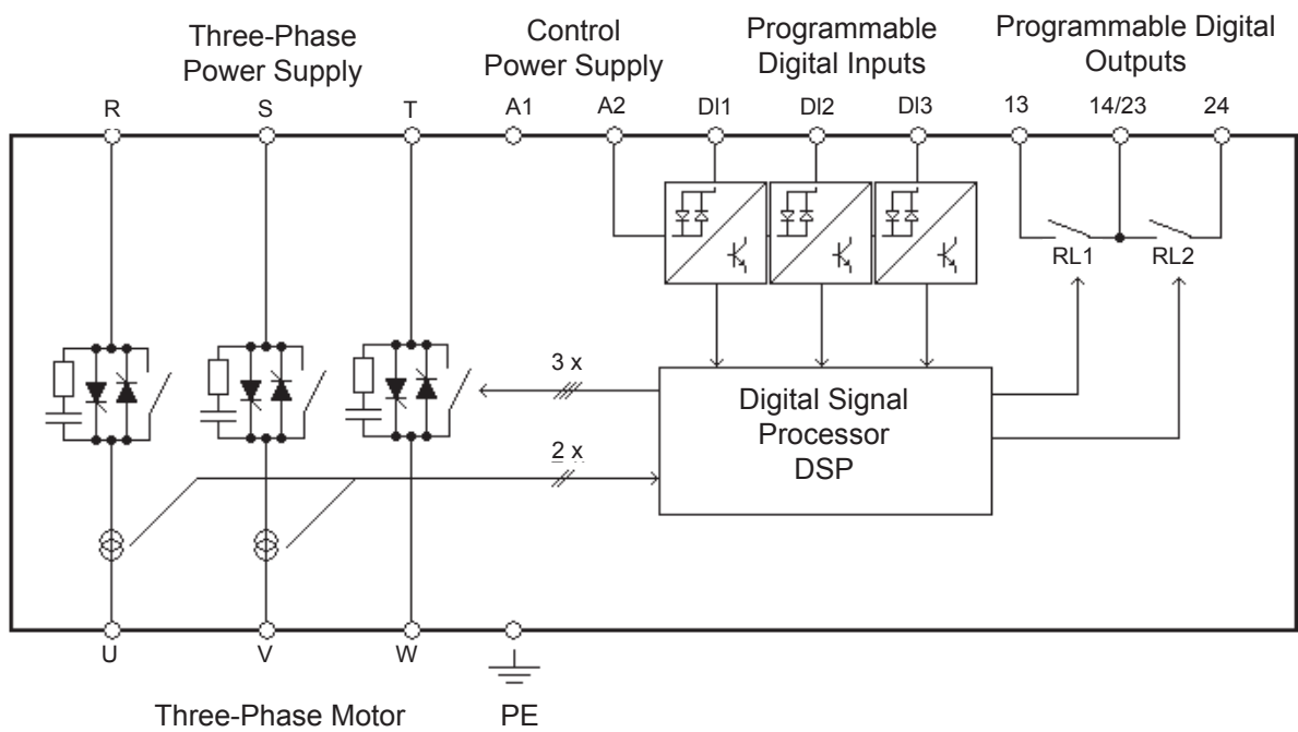
Figure 2.2 - Soft-Starter SSW-07 block diagram
