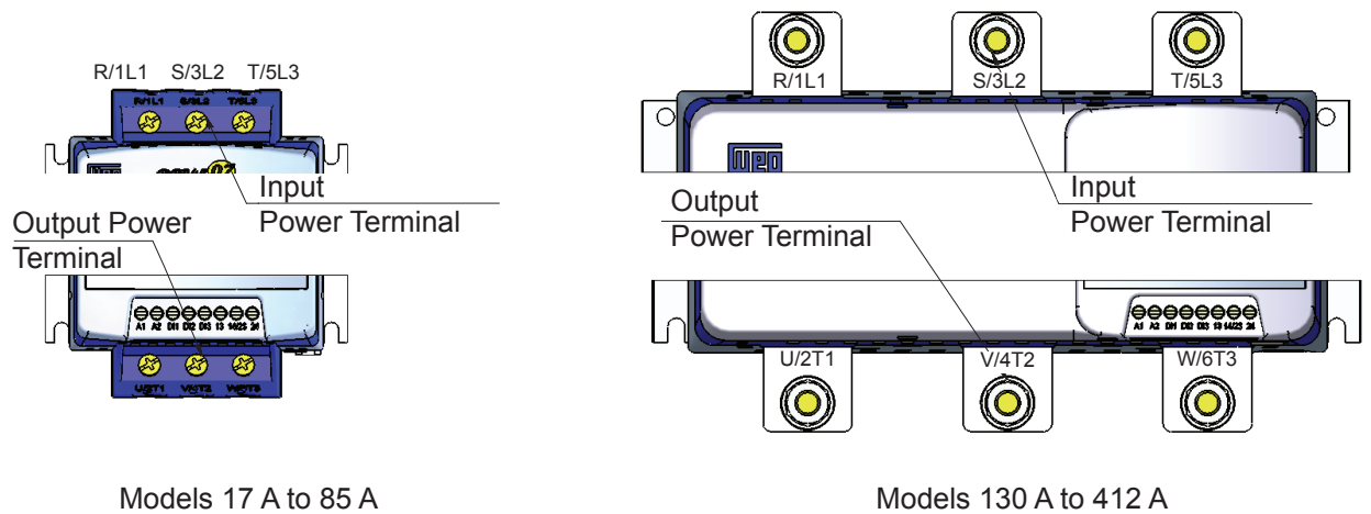
Figure 3.5 - Power terminals
