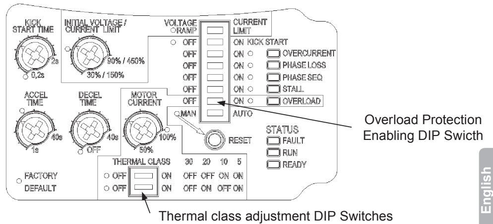
Figure 4.10 - Overload protection Enabling and Adjustment
