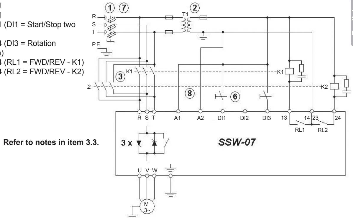
Figure 3.12 - Recommended Set-up with Command via Two-wire Digital Inputs and Direction of Rotation
