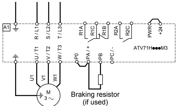
Connecting to the Altivar 71
