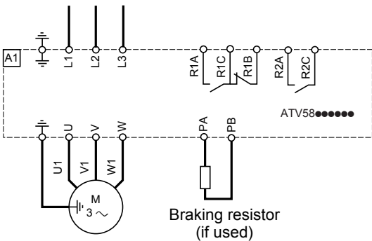
Connecting to the Altivar 58
