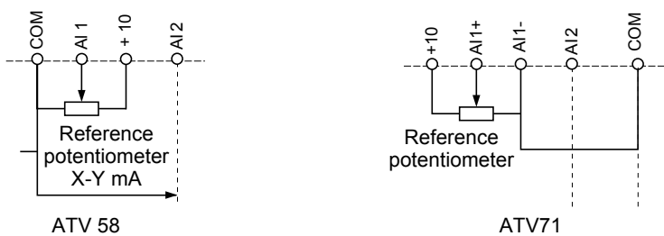
AI1 input on the ATV 71 wired as non differential 0-10 V (same as AI1 on the ATV58)
