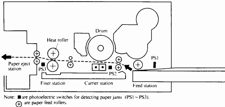
Figure 3.7 Paper path and paper sensors
