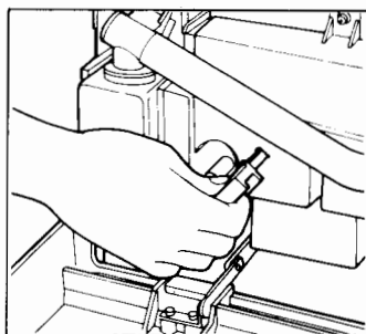
Figure 3.7 Replacing the oil felt
