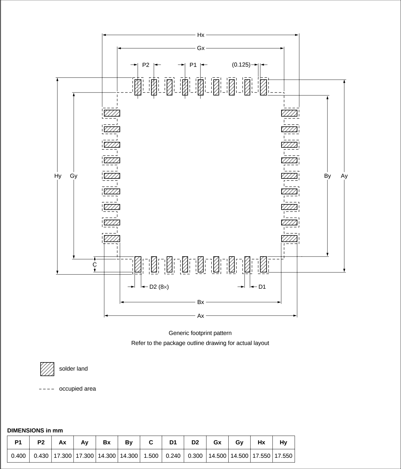
Footprint information for reflow soldering of LQFP128 package
