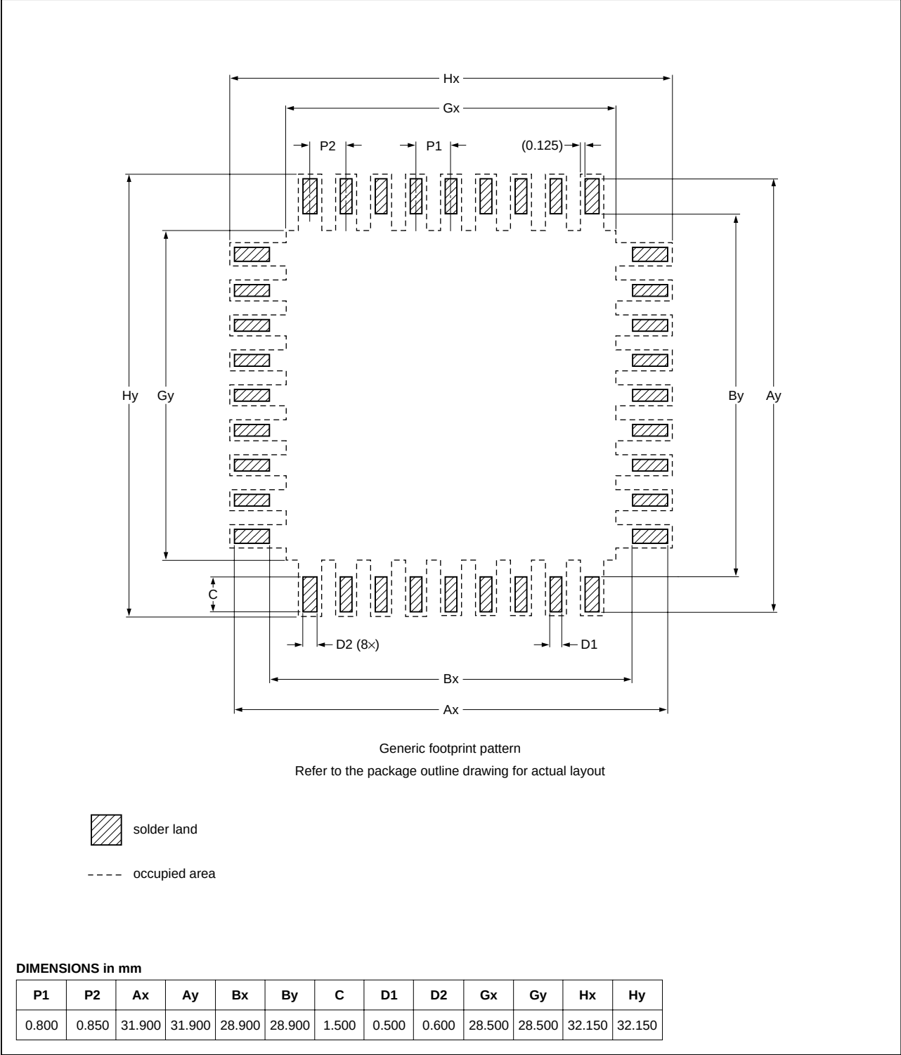
Footprint information for reflow soldering of QFP128 package
