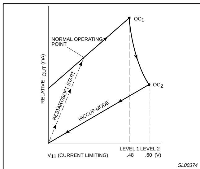
Figure 15. Output Characteristics
