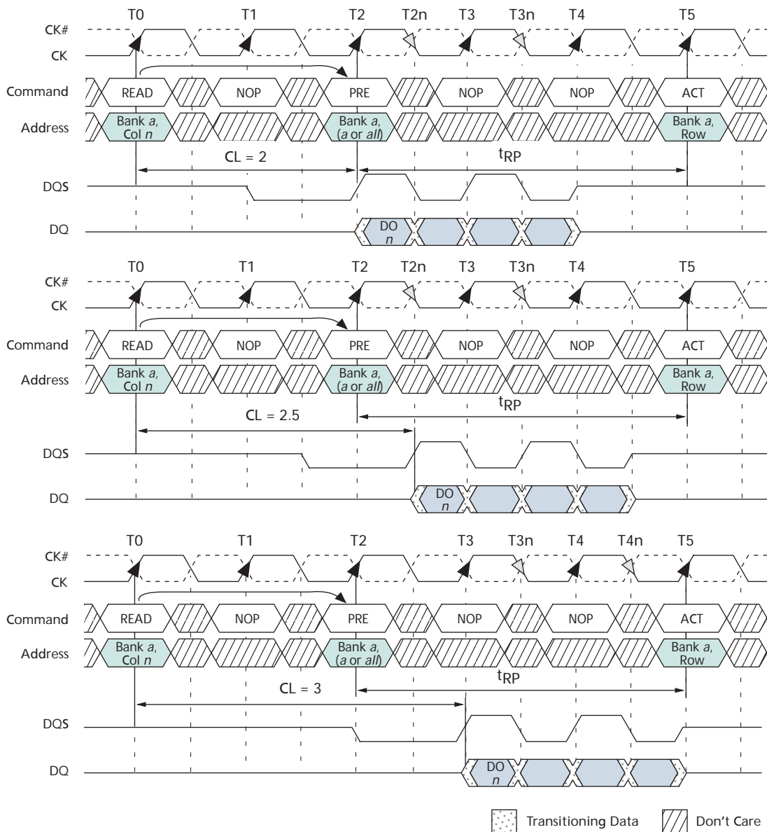
Figure 34: READ-to-PRECHARGE
